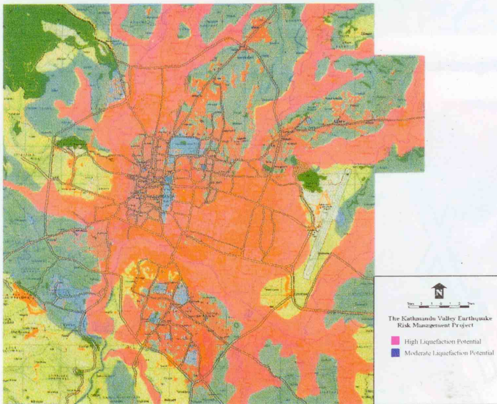
Figure 2. Liquefaction potential in Kathmandu and Lalitpur
