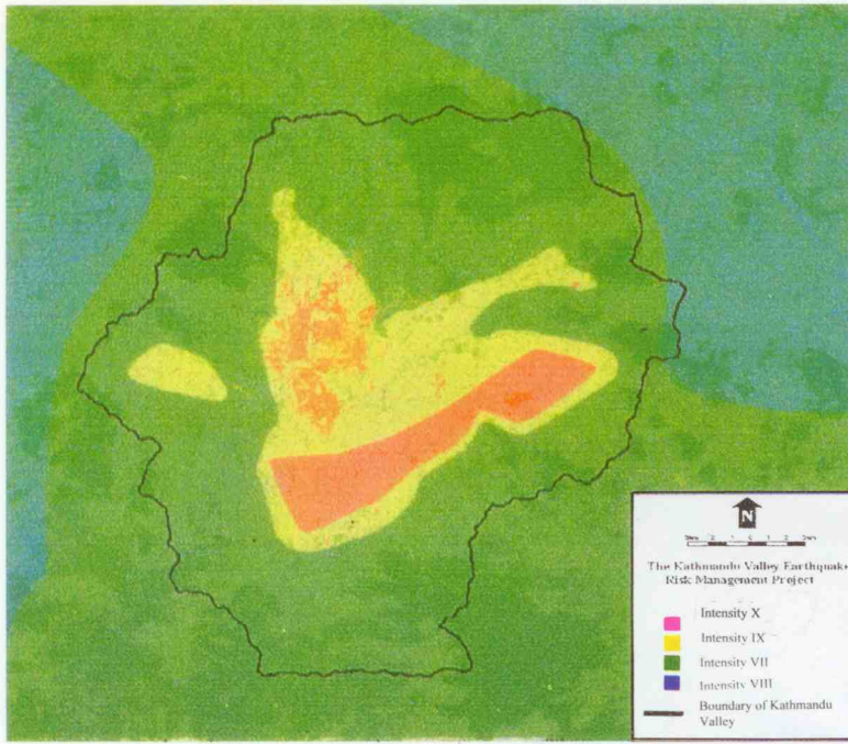
Figure 1. Modified Mercalli Intensity distribution from 1934 Earthquake
